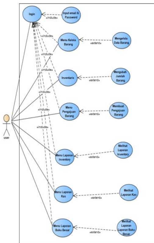
Gambar .III Use case Halaman User
